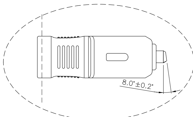
SC/APC Angles(SCALE 2/1)
