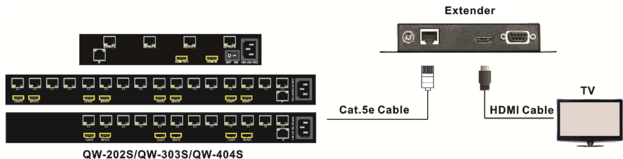
Figure 45: Extender Connection
