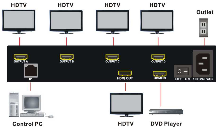
Figure 17: QW-202H Connections
