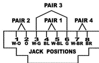
Figure 15: LAN Connector
