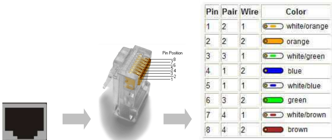
Figure 25: LAN (HDBT) Port Pin Definition
