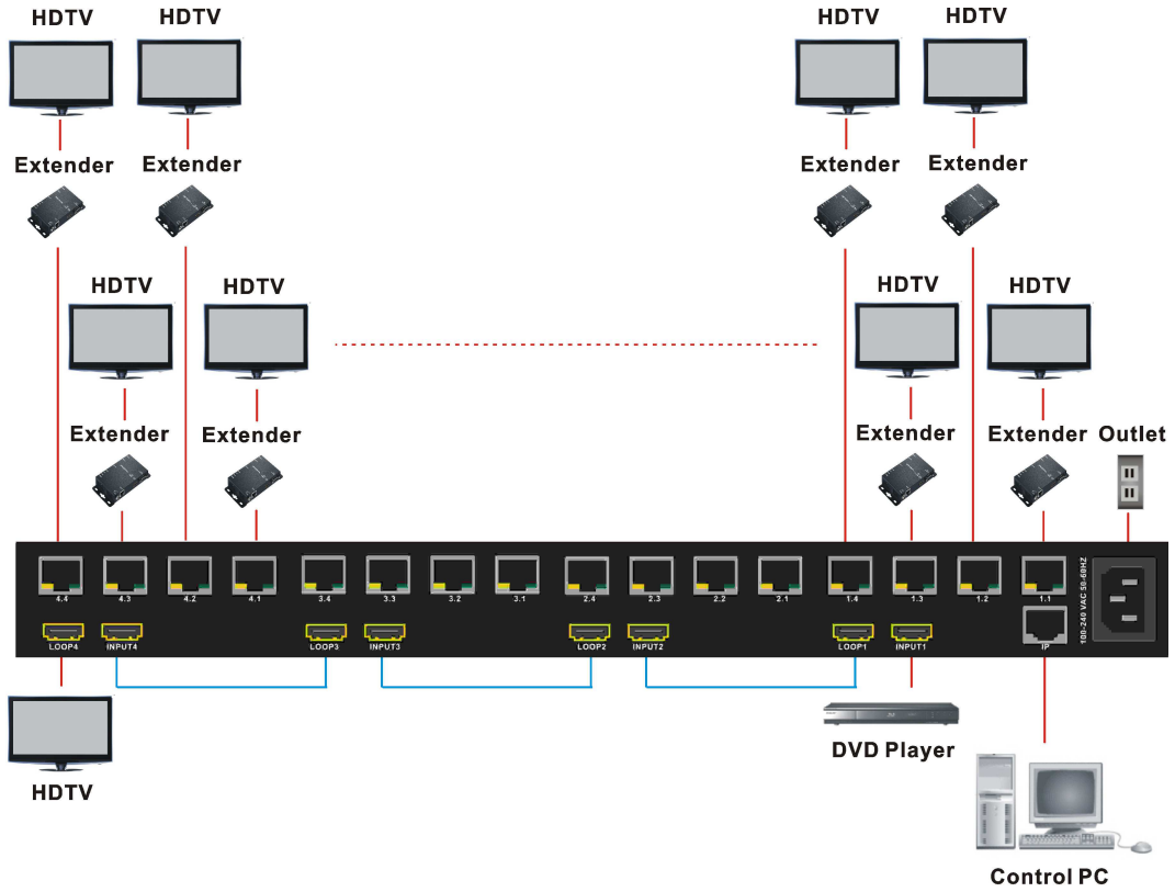
Figure 20: QW-404S Connections
