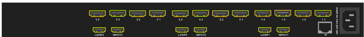
Figure 11: QW-303H Rear Panel
