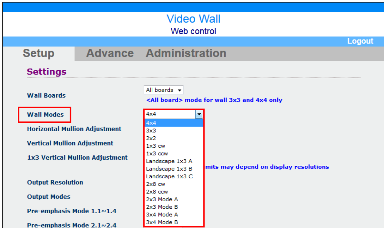
Figure 46: Wall Modes List for QW-404x
