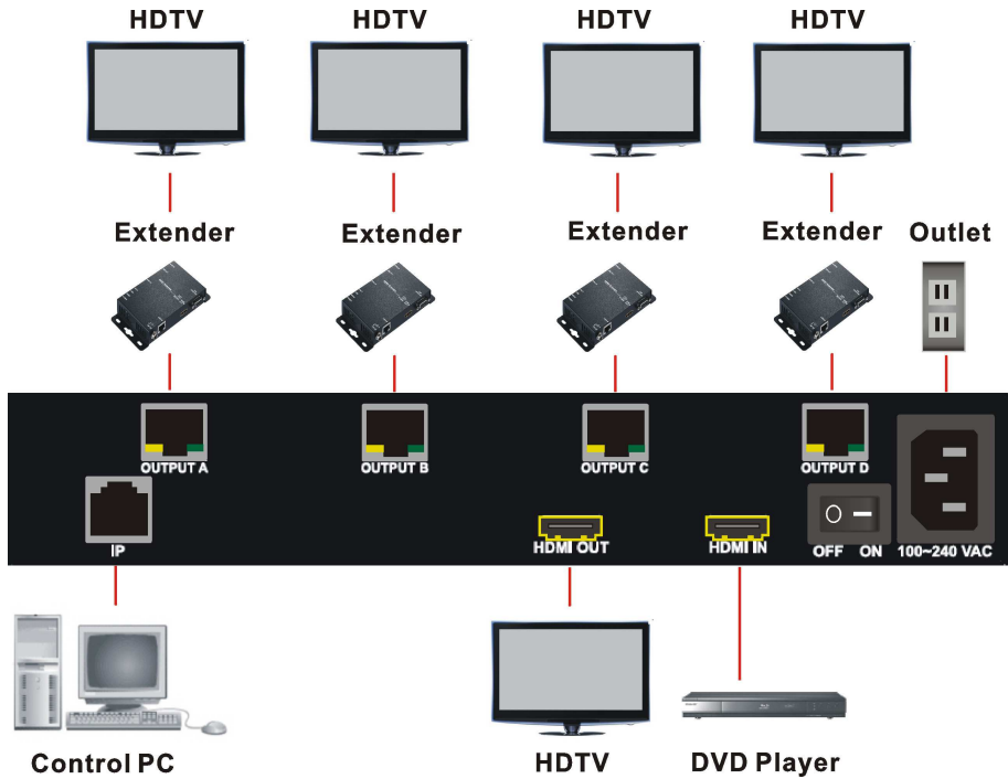
Figure 16: QW-202S Connections
