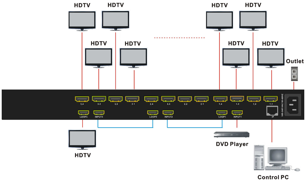
Figure 19: QW-303H Connections
