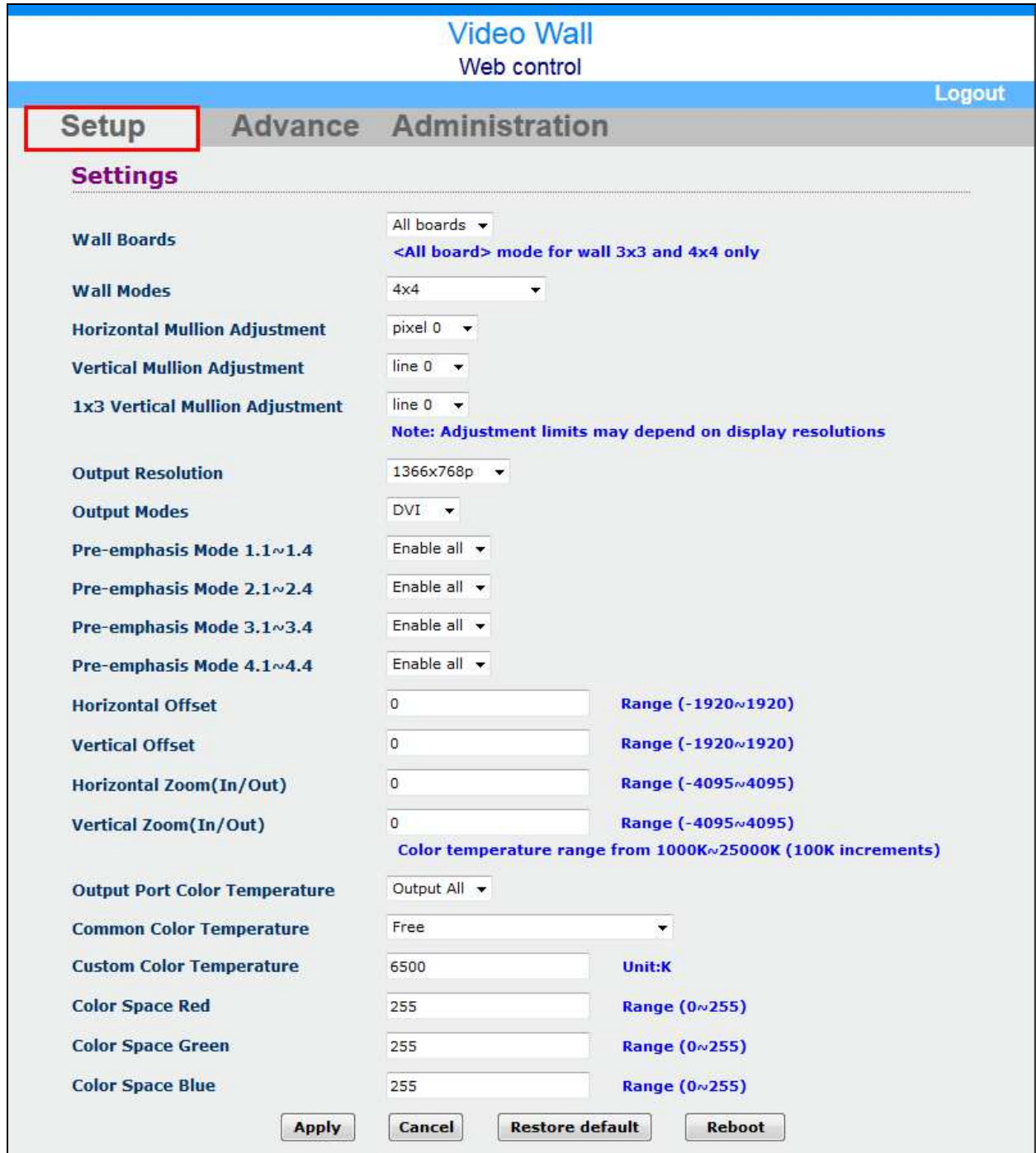
Figure 30: Web Control - Setup
