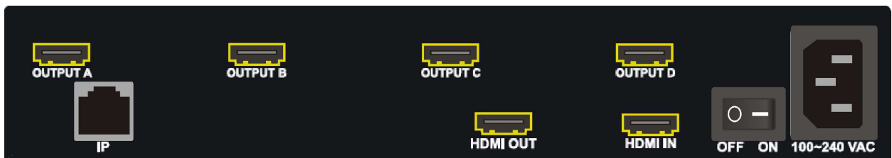
Figure 9: QW-202H Rear Panel
