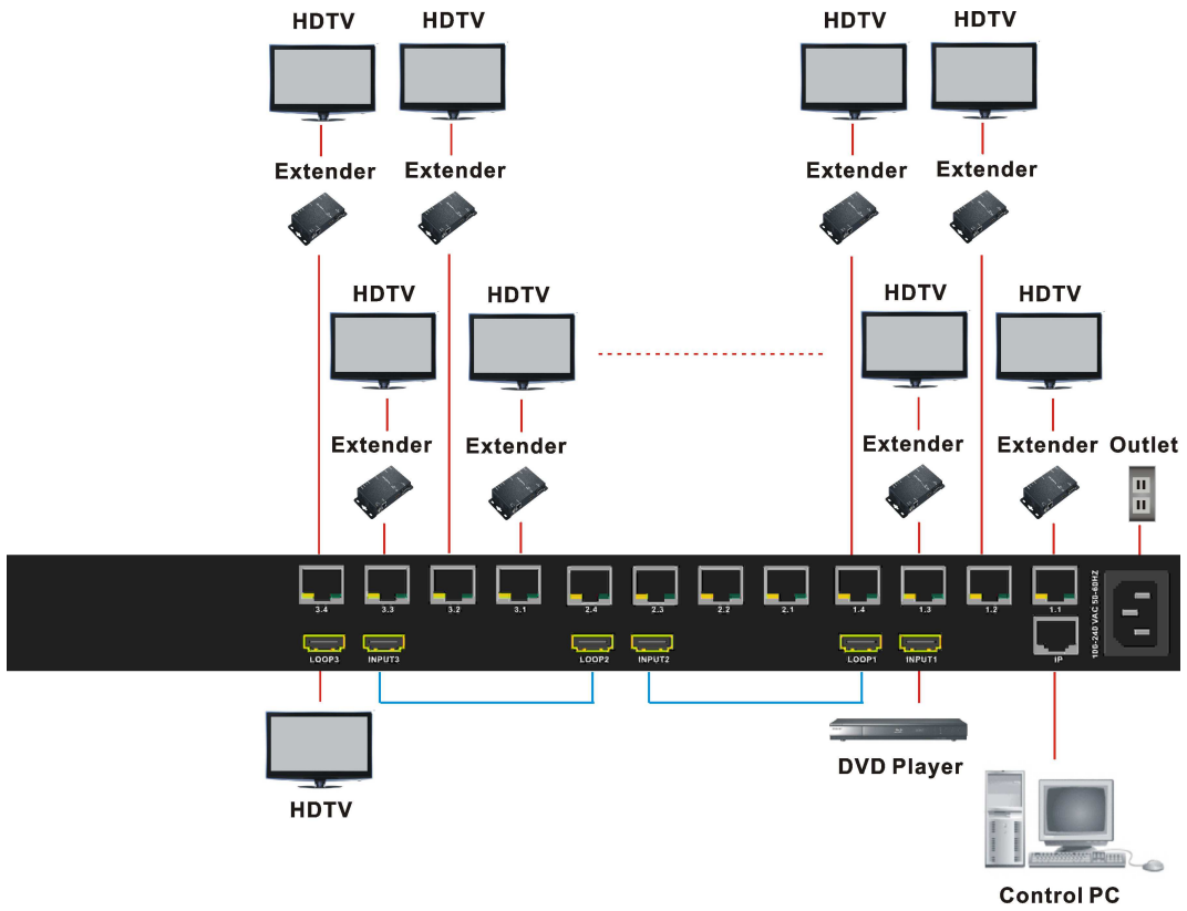
Figure 18: QW-303S Connections
