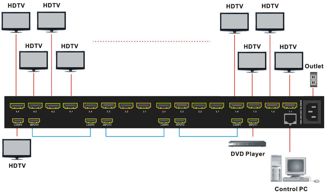
Figure 21: QW-404H Connections
