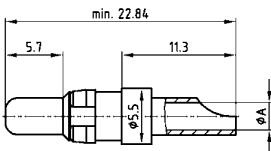
Plug contact
