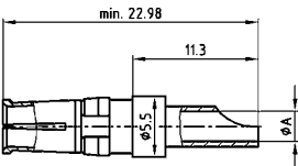
Socket contact
