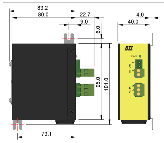
Panel & wall mount Dimension
