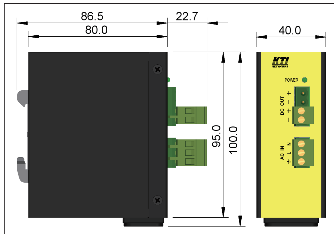
DIN-Rail mount Dimension
