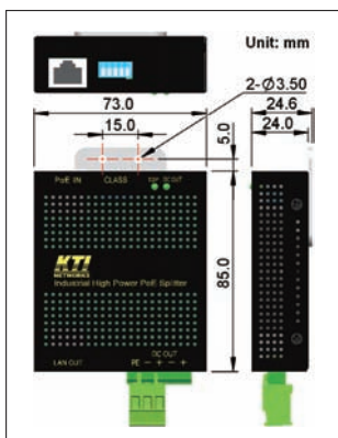
Panel Dimension
