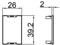
Blank module cover 2PCS
