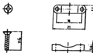
LOCK SCREW
