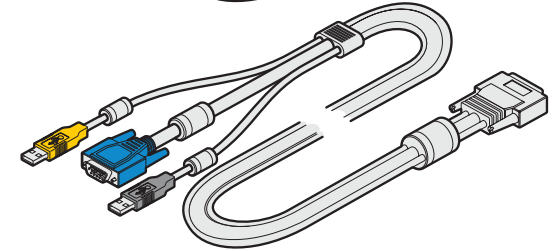
Shielded link cable (VGA, USB keyboard/mouse, USB card reader) Part code: VSCD6 (length 1.8m/6ft)
