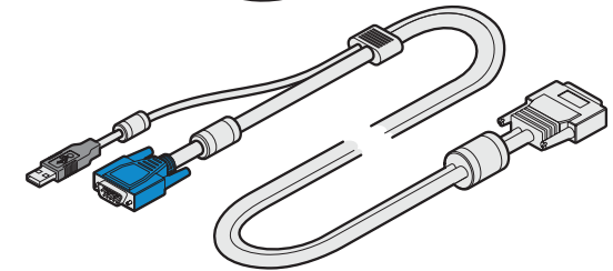
Shielded link cable (VGA, USB keyboard/mouse) Part code: VSCD7 (length 1.8m/6ft)
