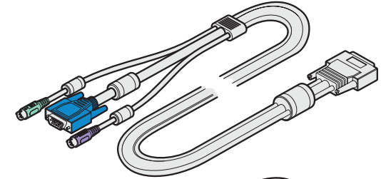
Shielded link cable (VGA, PS/2 keyboard, PS/2 mouse) Part code: VSCD5 (length 1.8m/6ft)
